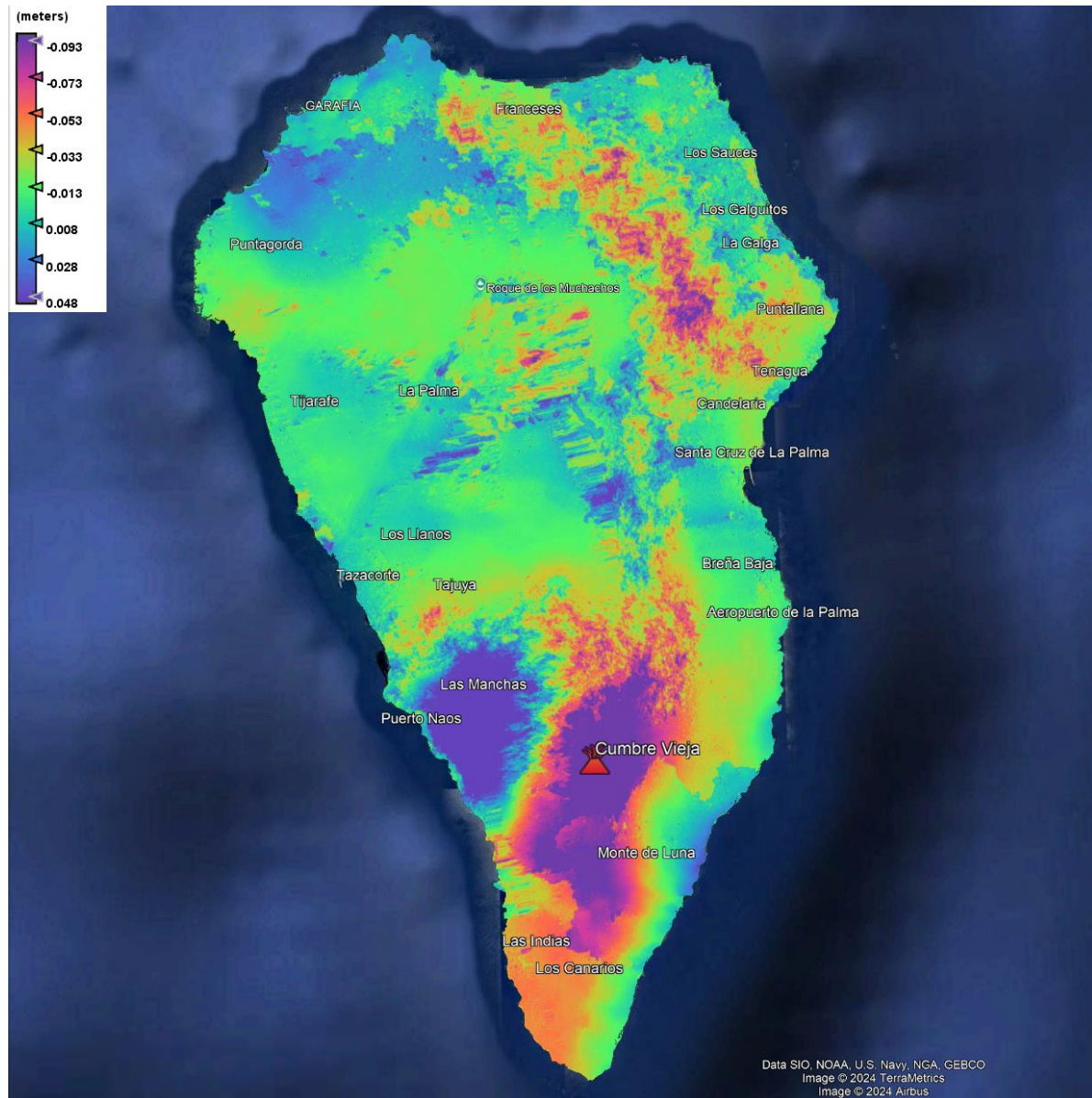
Figure 27. Displacement map of the study area, visualized in GoogleEarth Pro.
