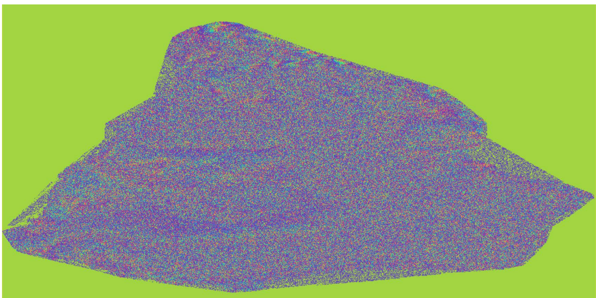
Figure 14. Differential interferogram after the Topographic Phase Removal.
