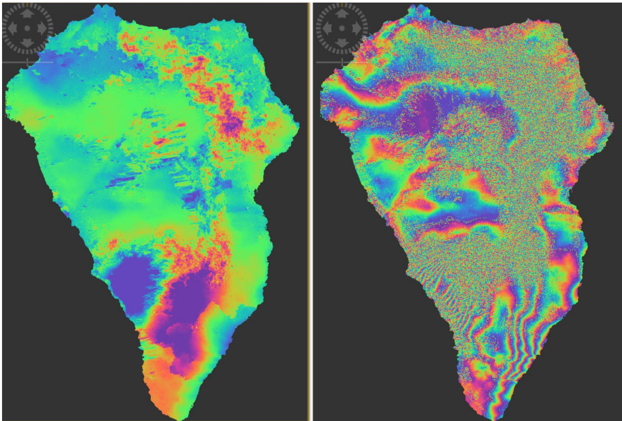
Figure 26. Comparison of the georeferenced displacement map (left) and the differential interferogram (right).
