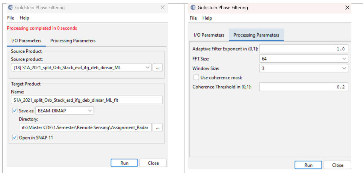
Figure 17. Goldstein Phase Filtering.
