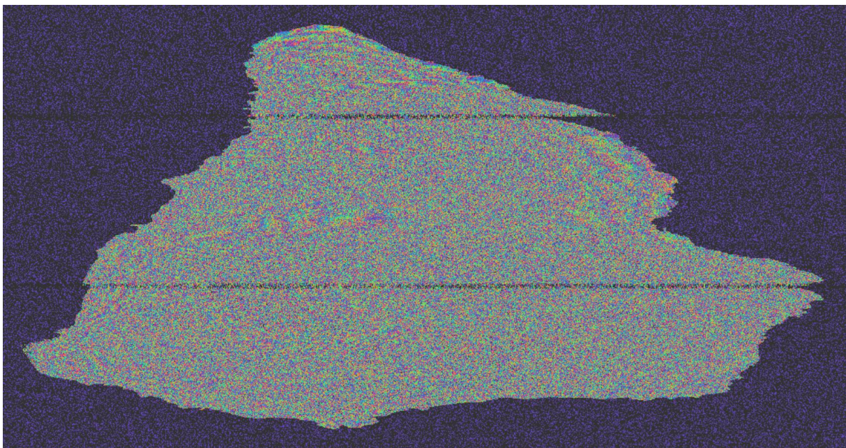
Figure 10. Topographic interferogram produced with the Sentinel-1 SLC images of the pre- and post-event.
