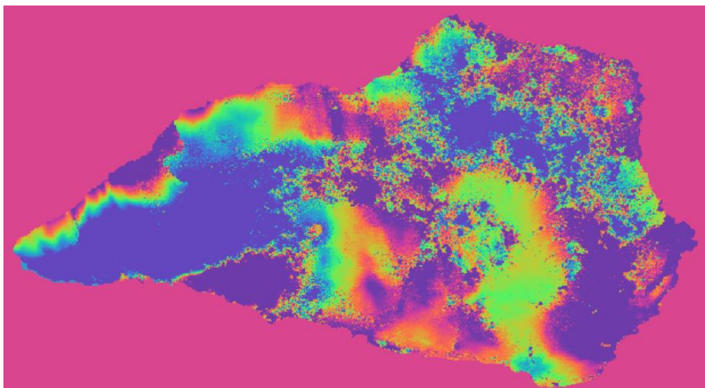
Figure 21. Unwrapped Phase of the study area.
