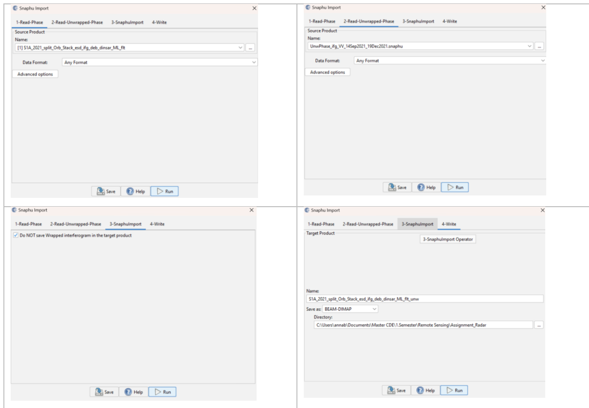
Figure 20. Importing the phase which was unwrapped with Snaphu in the console into SNAP.
