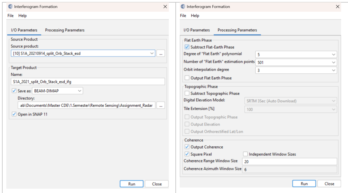
Figure 9. Interferogram Formation tool.
