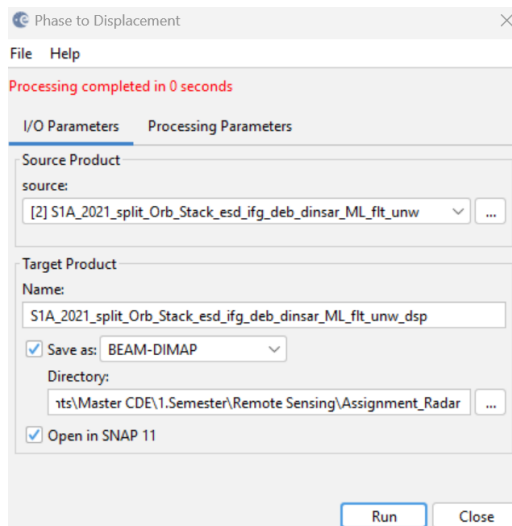
Figure 22. Phase to Displacement tool to generate a displacement map.
