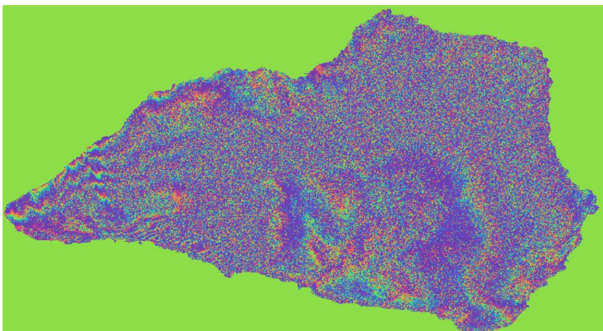
Figure 16. Differential interferogram with improved visual interpretability after using the Multilooking tool.
