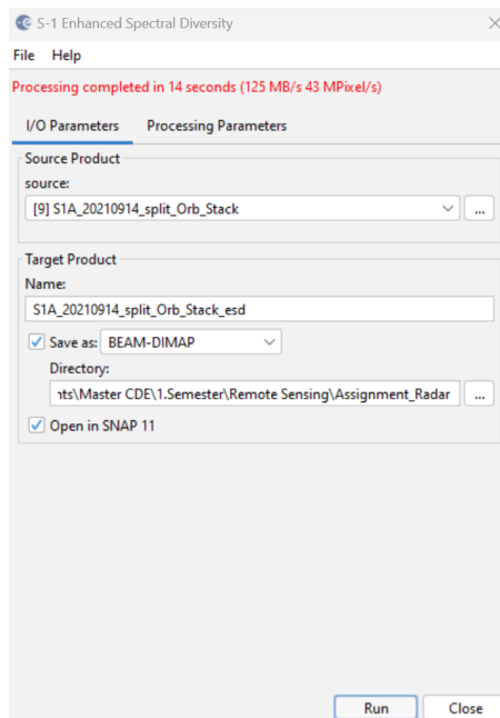
Figure 7. S-1 Enhanced Spectral Diversity tool.
